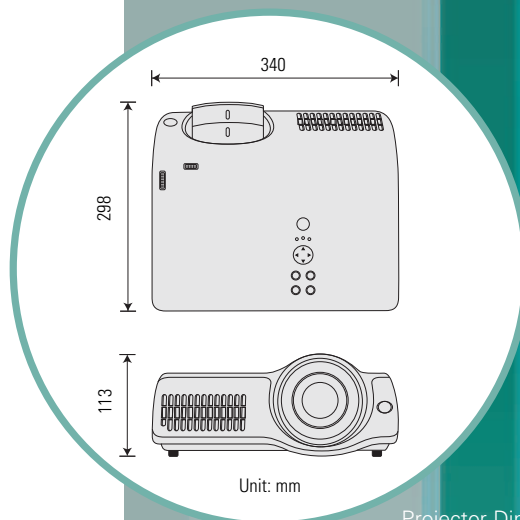
Projector Dimensions
