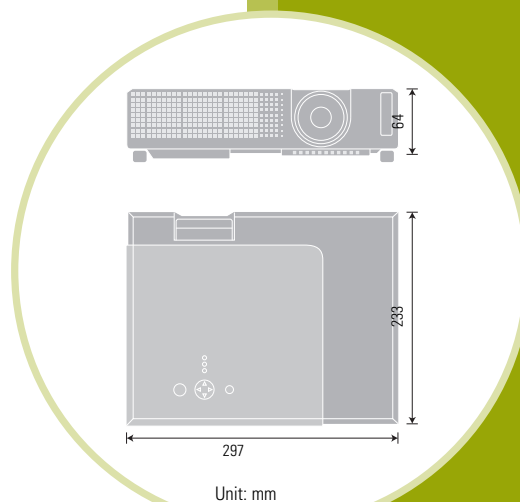
Projector Dimensions
