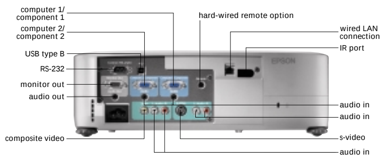
Back view PowerLite 830p
